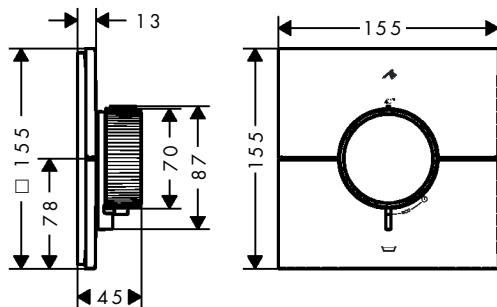
AXOR ShowerSelect ID square 36753XX0
