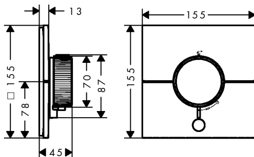
AXOR ShowerSelect ID square 36777XX0
