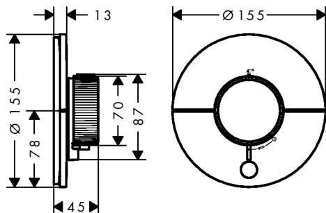
AXOR ShowerSelect ID round 36776XX0
